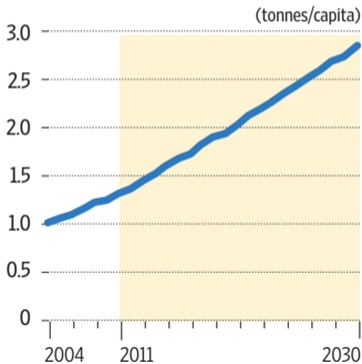
Per capita CO 2 emission: reference scenario
