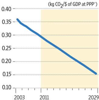
CO 2 emission intensity under reference scenario
